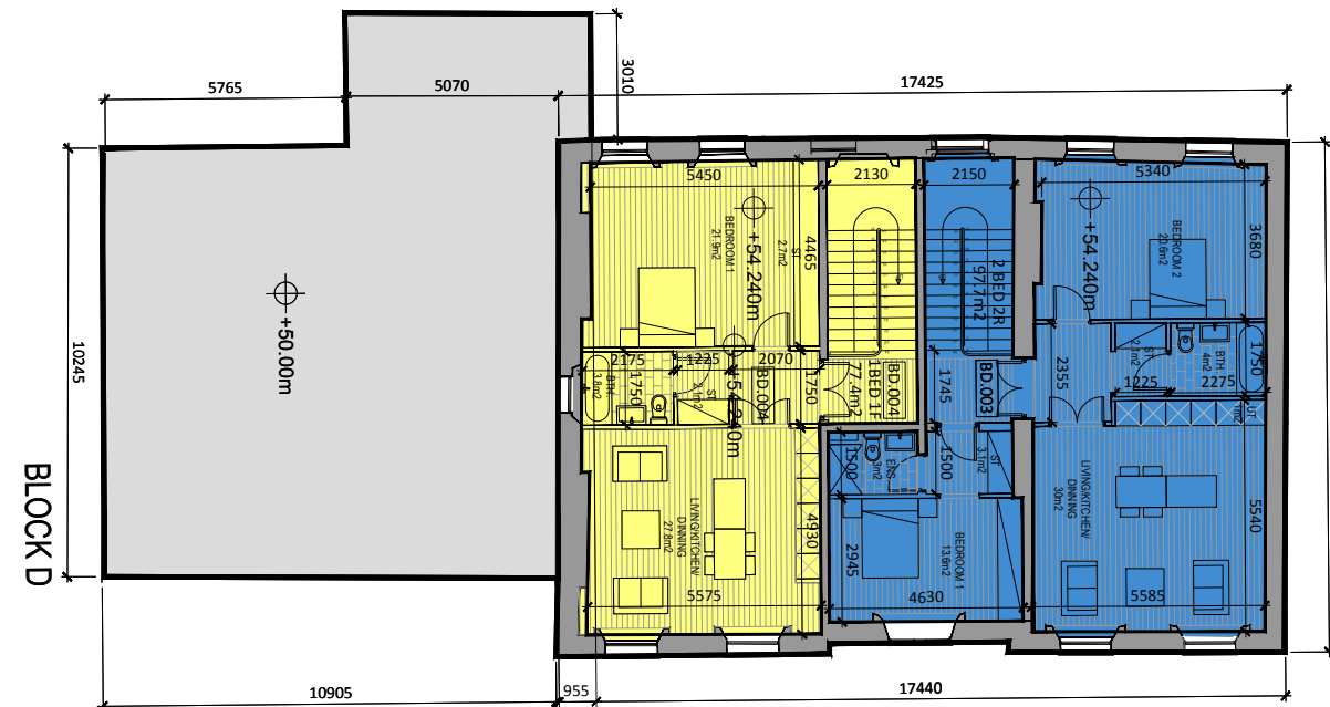
FIRST FLOOR PLAN ESC: 1/200
